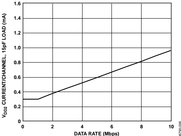
Figure 6. Typical Output Current per Channel vs. Data Rate (15 pF Output Load)
